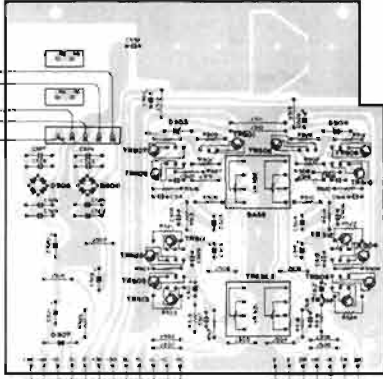
POWER C BOARD NA07153 (U: NA07154)
